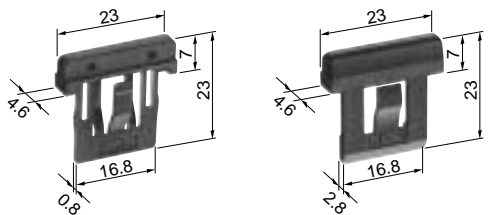
Center Barrier for Guard Cover
