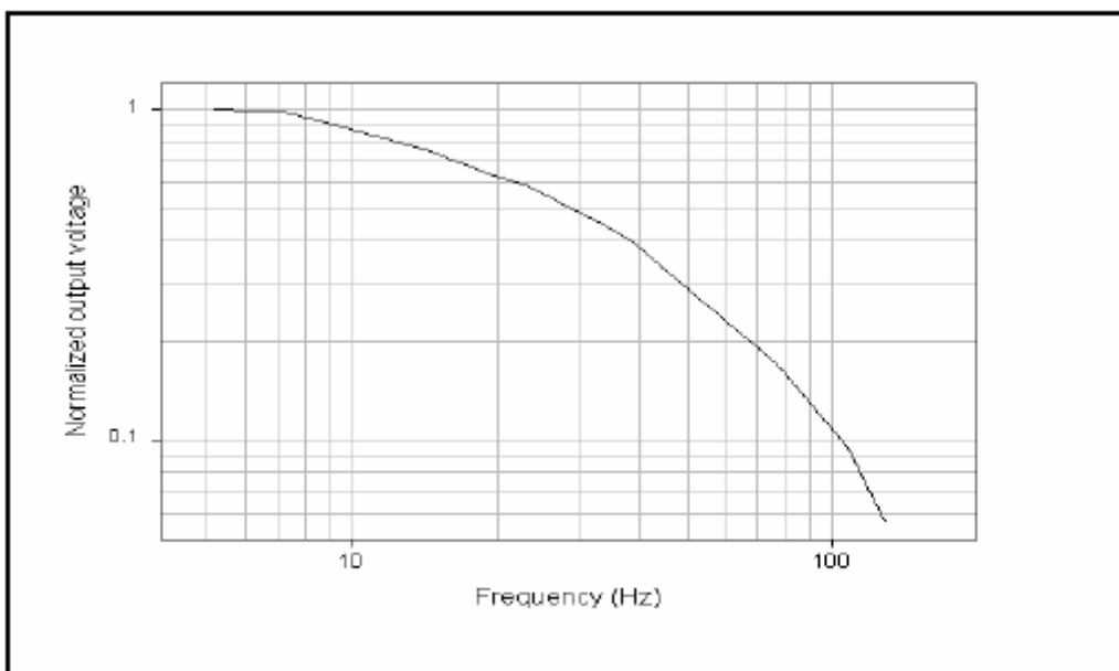
Figure 2: Frequency response
