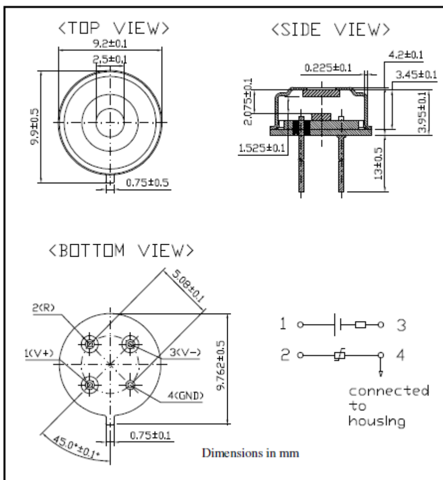
Figure 5: Mechanic drawing and pin assignment
