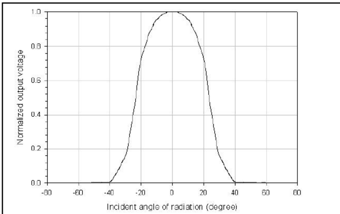
Figure 3: Field of view curve
