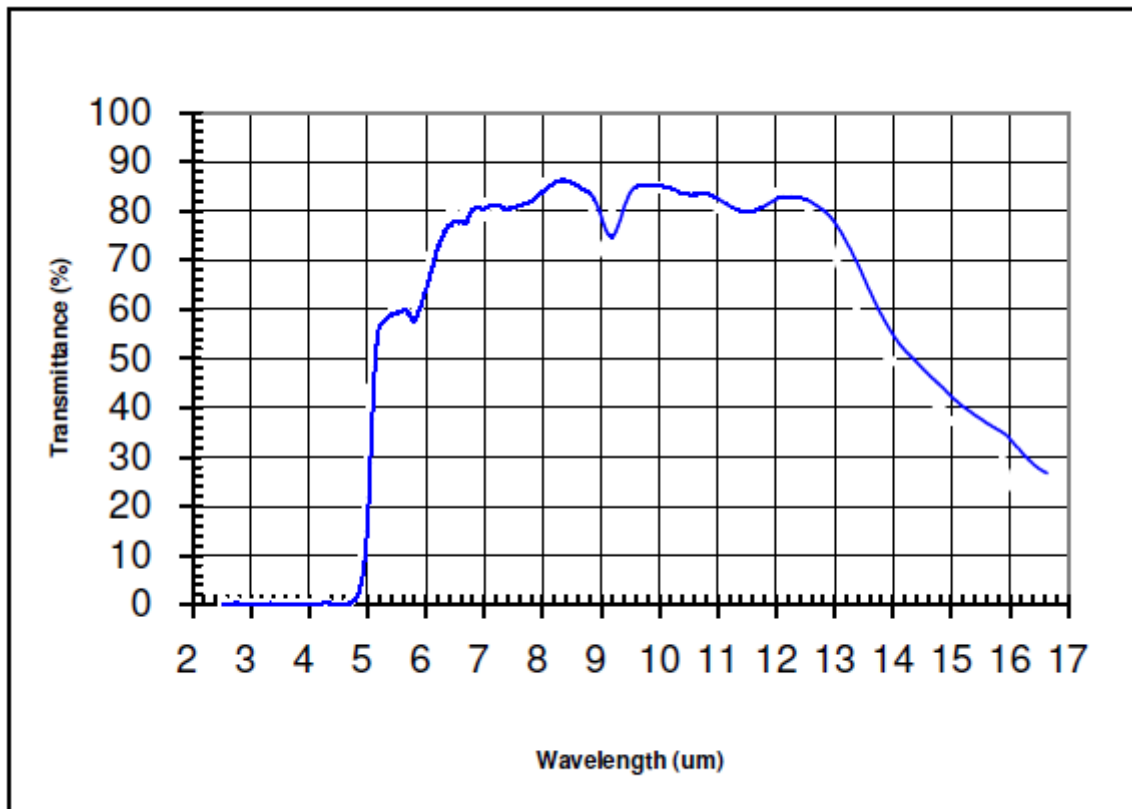
Figure 4: Typical spectral transmittance curve
