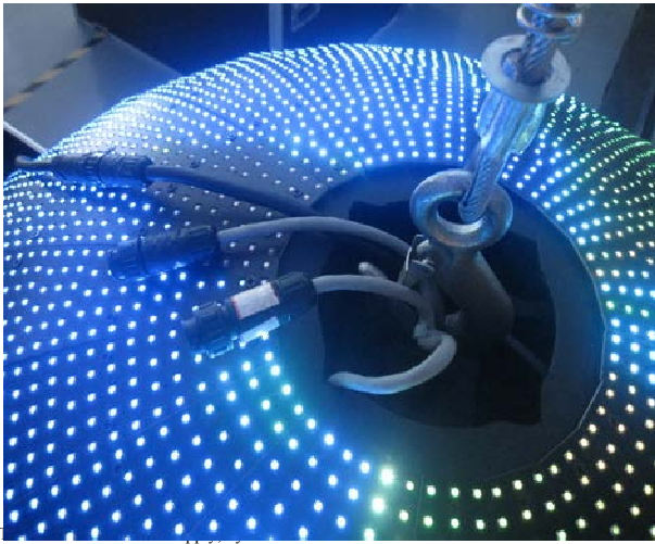
Asynchronous cable
