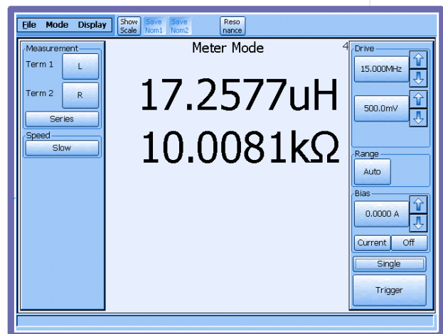
Example of measurement showing clear and concise digital display of component characteristics
