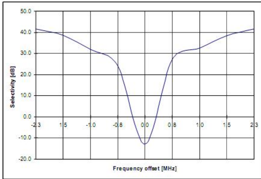
Selectivity at 250K Baud Data Rate
