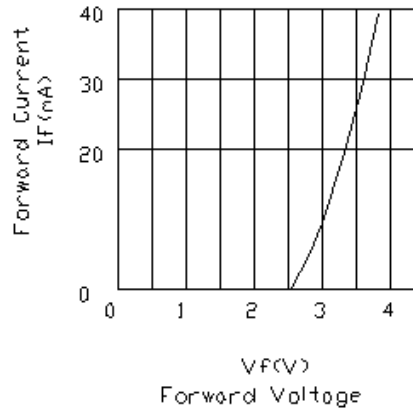
A LED Forward Current VS. — Forward Voltage
