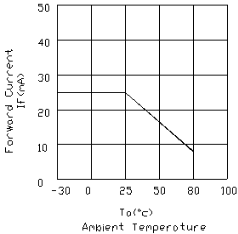
A LED Forward Current VS. — Ambient Temperature
