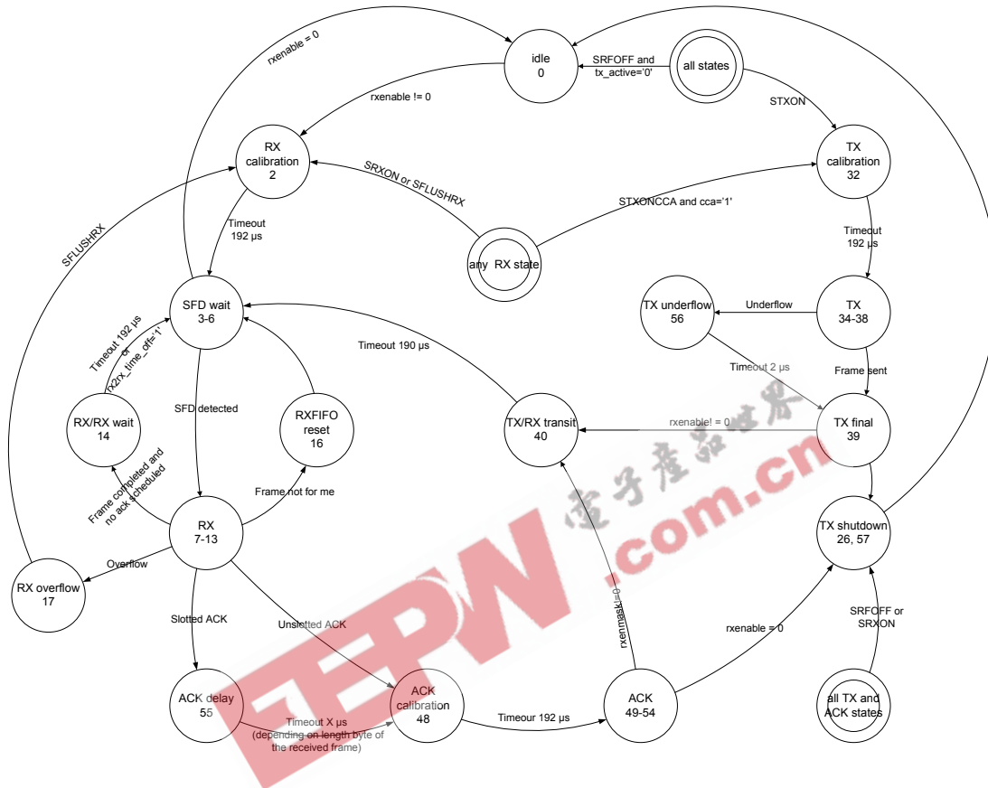
Figure 30: Main FSM
