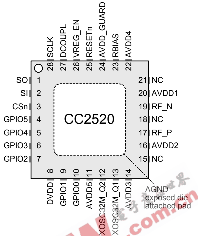
Figure 1: Pinout of CC2520 (top view)
