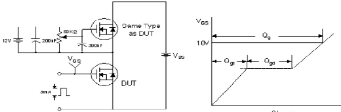
Gate Charge Test Circuit and Waveform
