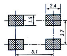
Figure 3) S X 7 - Recommended Solder Pad Layout, Top view
