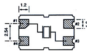
Figure 2) S X 7 - Pad Configuration Bottom view
