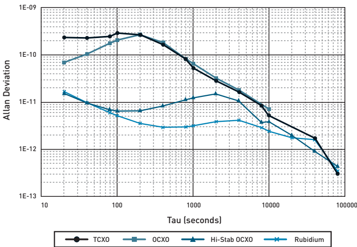
XL-GPS Disciplined Oscillator Allan Variance Example
