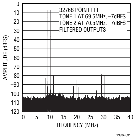
70MHz 2-Tone 32768 Point FFT LT1993-4 Driving LTC2249 14-Bit ADC
