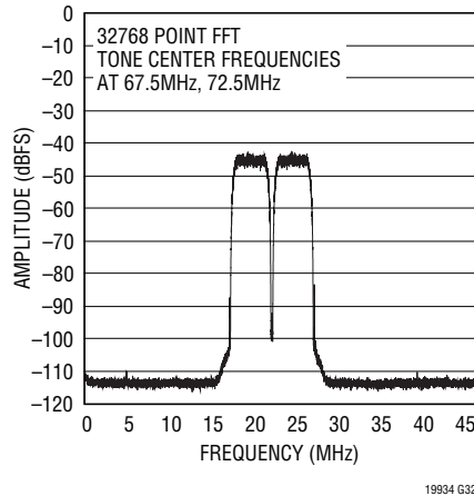
2-Tone WCDMA Waveform LT1993-4 Driving LTC2255 14-Bit ADC at 92.16Msps
