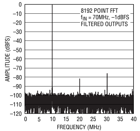
70MHz 8192 Point FFT, LT1993-4 Driving LTC2249 14-Bit ADC
