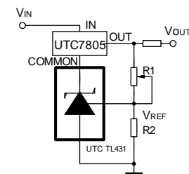
Output Control of a Three-Terminal Fixed Regulator
