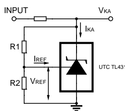
For V_{KA} = V_{REF} \cdot (1 + R1/R2) + I_{REF} \cdot R1
