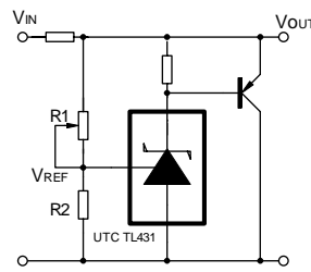
Higher-current Shunt Regulator
