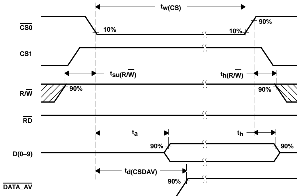
Figure 36. Read Timing Diagram Using R/\overline{W} ( \overline{CS0} -controlled)
