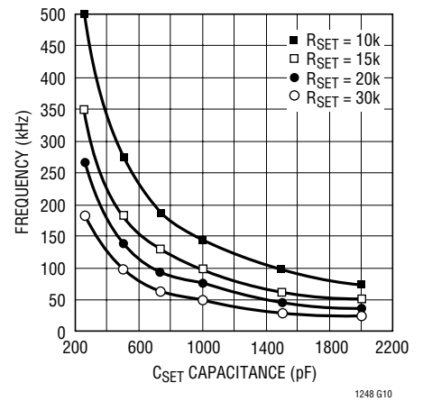
Frequency vs R_{SET} and C_{SET}
