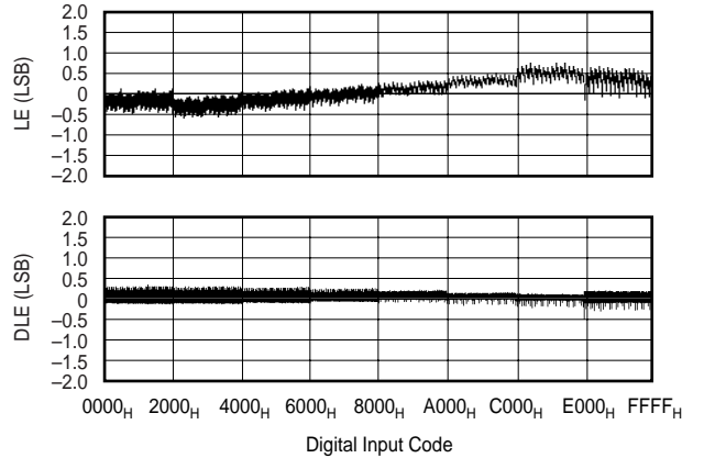
LINEARITY ERROR AND DIFFERENTIAL LINEARITY ERROR vs CODE (DAC B, +25°C)
