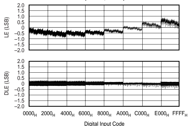
LINEARITY ERROR AND DIFFERENTIAL LINEARITY ERROR vs CODE (DAC B, +85°C)
