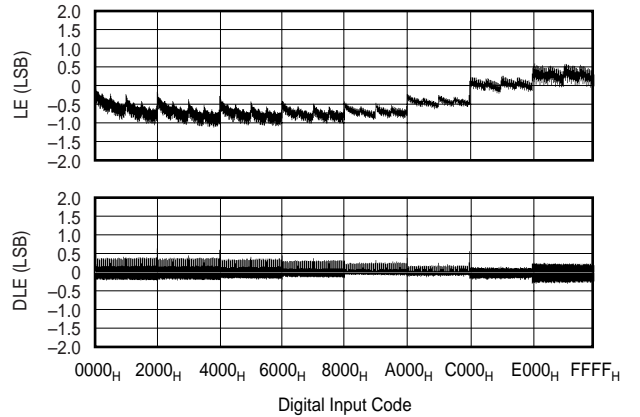
LINEARITY ERROR AND DIFFERENTIAL LINEARITY ERROR vs CODE (DAC D, +25°C)
