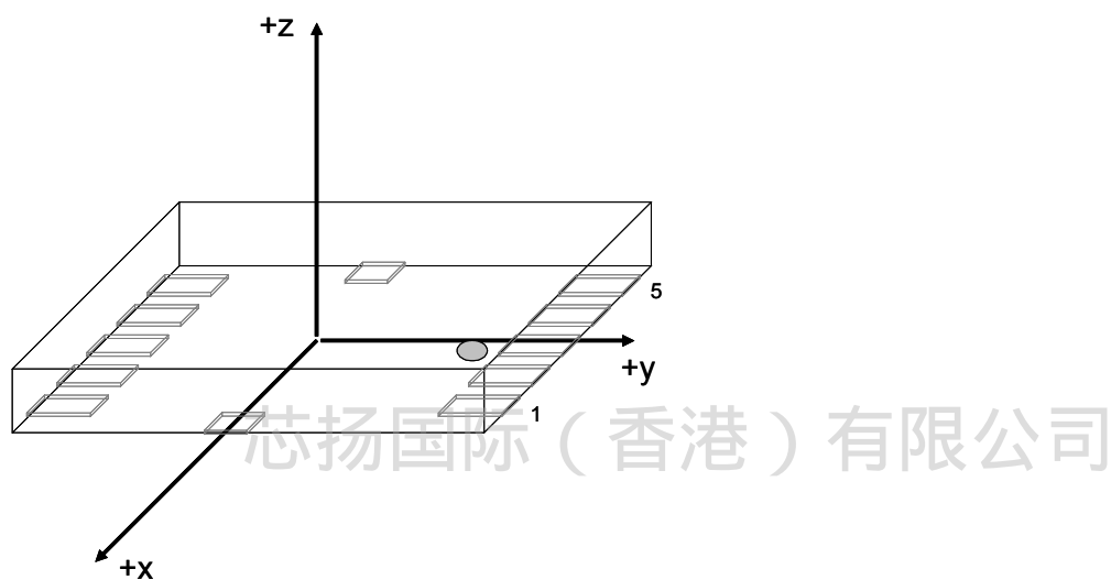
Figure 18: Axes orientation of the BMA023
