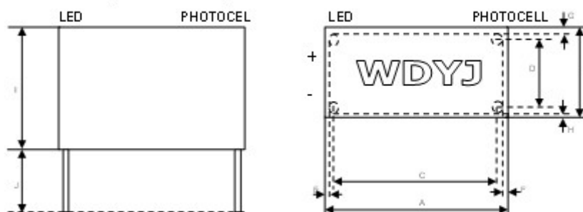
WDYJ-0202 series(CDS-LED Switch)
