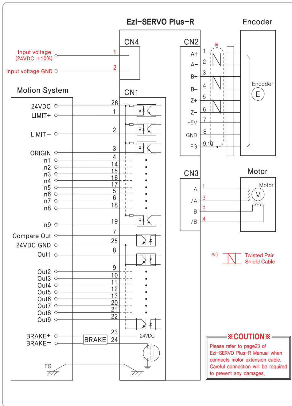
CONTROLLER EMBEDDED DRIVE EXTERNAL WIRING DIAGRAM
