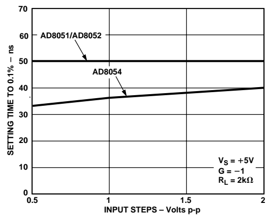
Figure 26. Settling Time vs. Input Step
