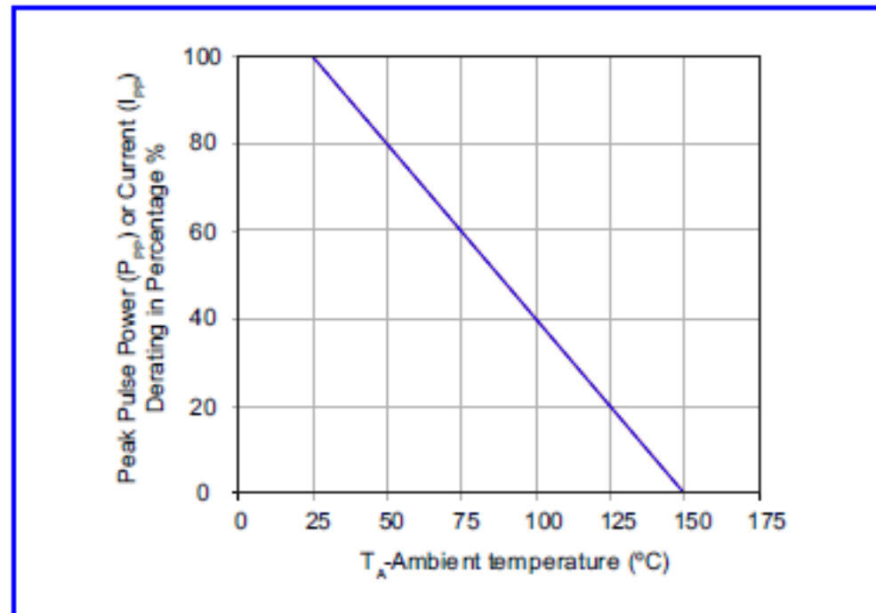
Figure 2 - Pulse Derating Curve
