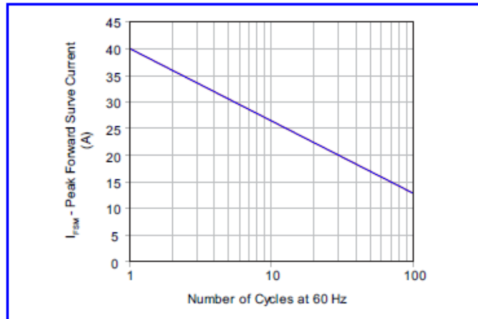
Figure 6 - Maximum Non-Repetitive Forward Surge Current Uni-Directional Only
