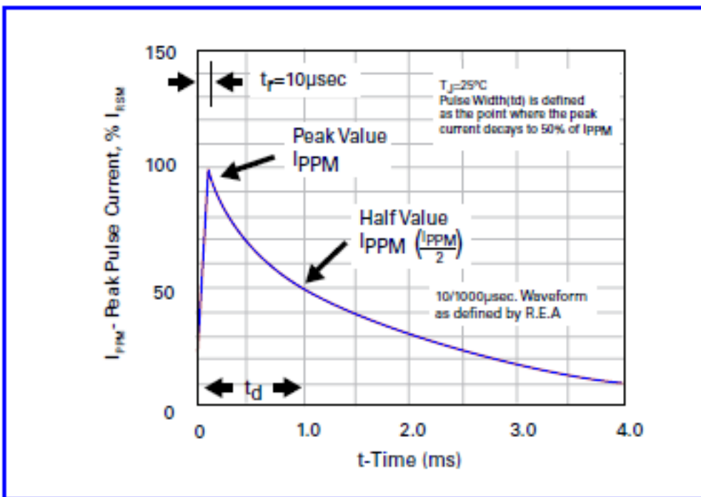
Figure 3 - Pulse Waveform
