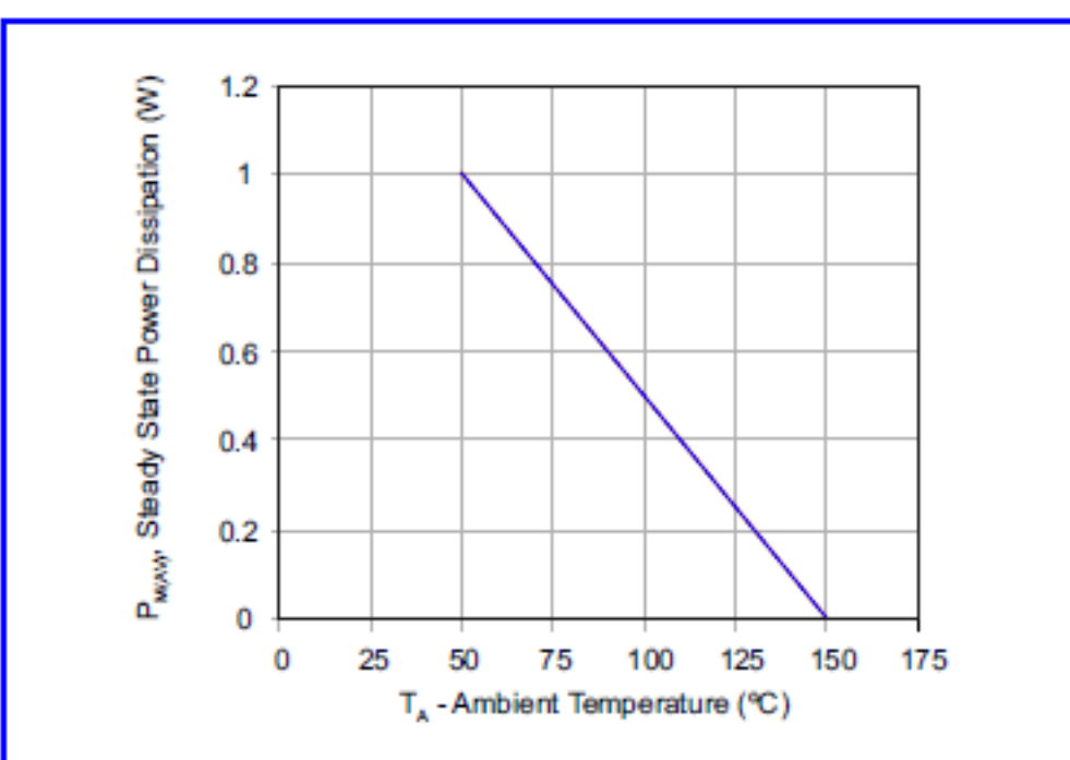
Figure 5 - Steady State Power Dissipation Derating Curve
