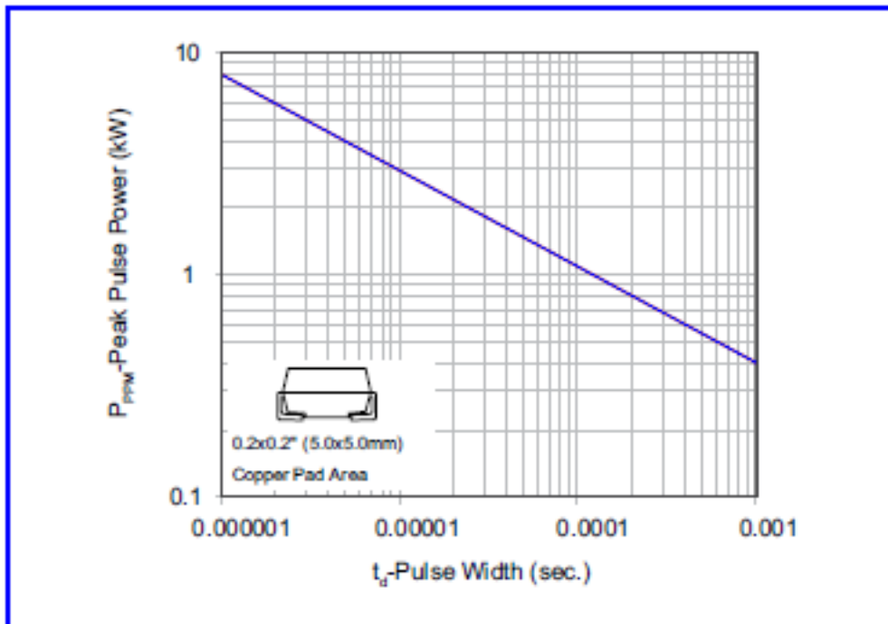
Figure 1 - Peak Pulse Power Rating Curve
