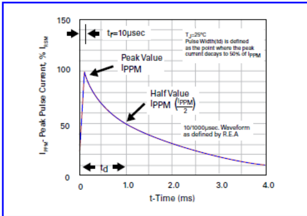
Figure 3 - Pulse Waveform
