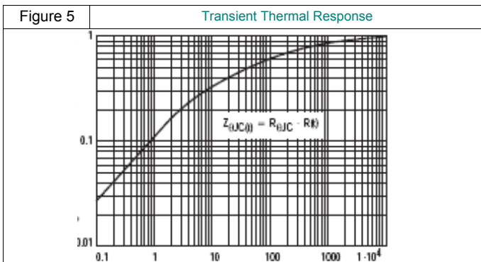
R(t) TRANSIENT THERMAL R(NORMALIZED); t , TIME(ms)
