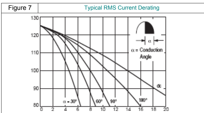
T_C , CASE TEMPERATURE(°C); I_{T(RMS)} , RMS ON-STATE CURRENT (AMPS)
