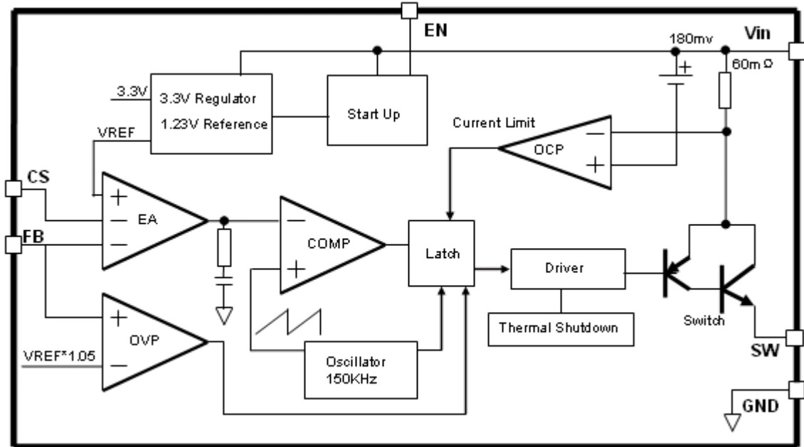
Figure3. Function Block Diagram of LPD3202
