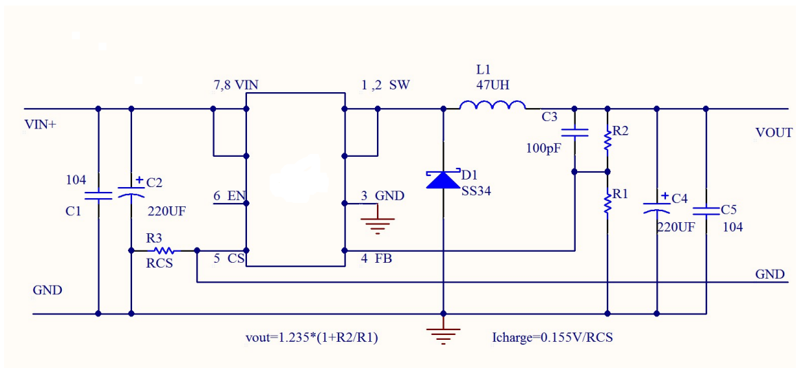
Figure4.LPD3202 Typical Application Circuit (Li Battery Charger)
