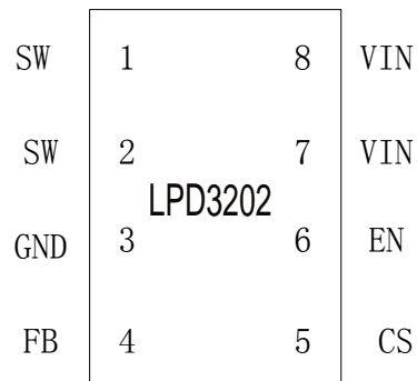
Figure2. Pin Configuration of LPD3202 (Top View)
