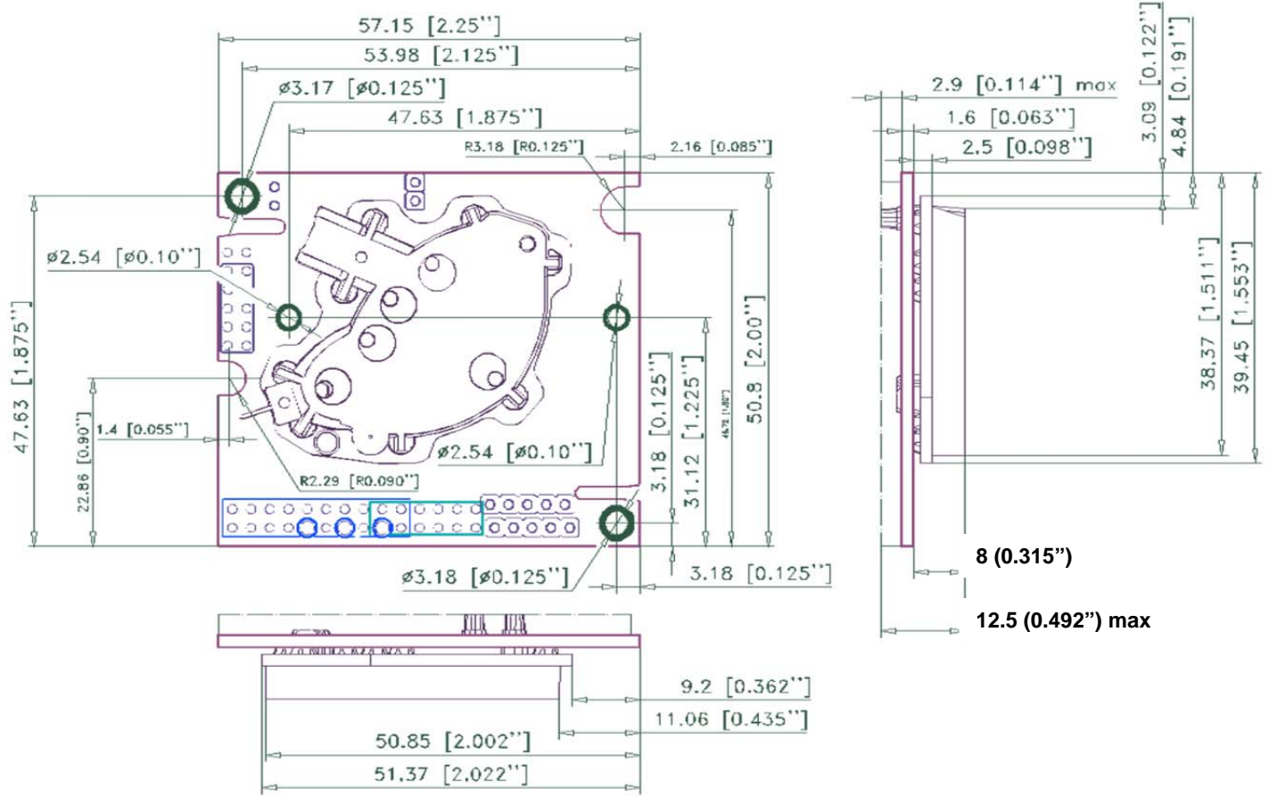
Figure 4. CO 2 Engine® K30 mechanical drawing.
