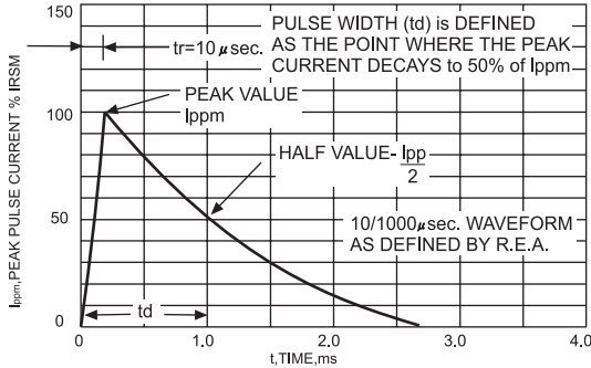
FIG.3-PULSE WAVEFORM
