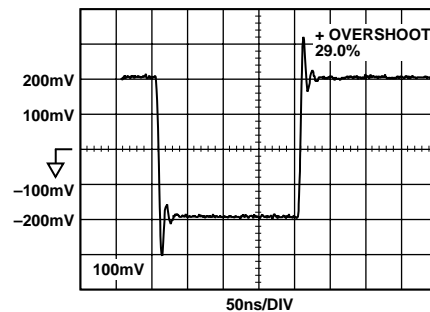
Figure 41. Typical Pulse Response with C_L = 65 pF, Gain = +2, and V_S = \pm 2.5 V
