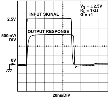
Figure 27. Input Overload Recovery, V_S = \pm 2.5\text{ V}
