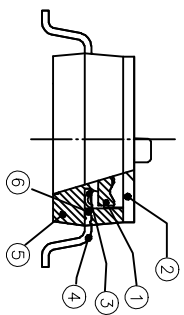
(Construction)
