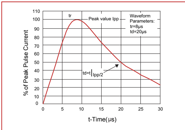
Figure 2. Pulse Waveforms
