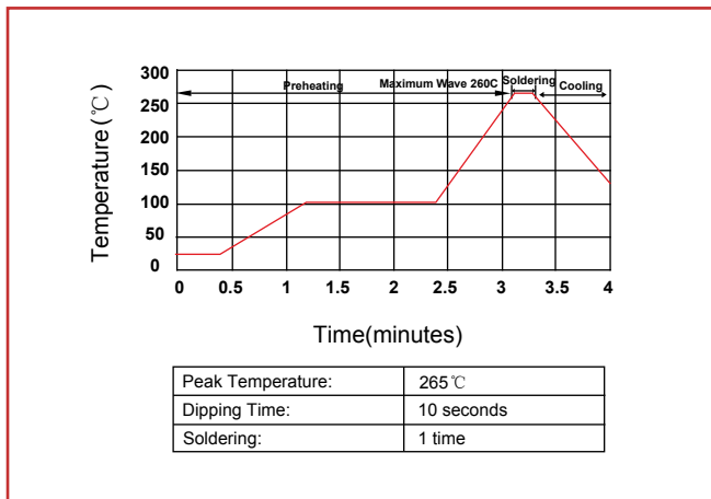
Figure 3. Flow / wave Soldering
