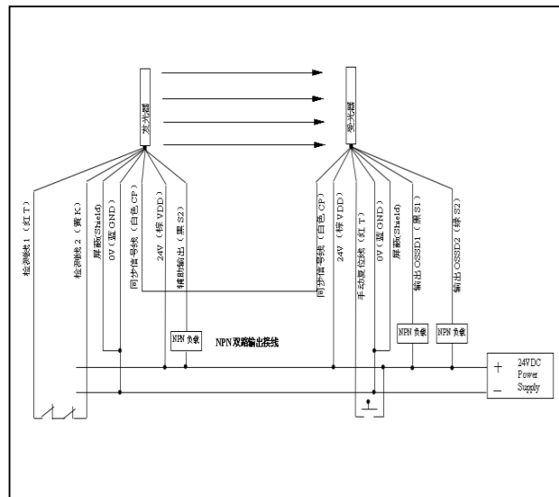
NPN输出接线图 The wiring diagram of NPN output
