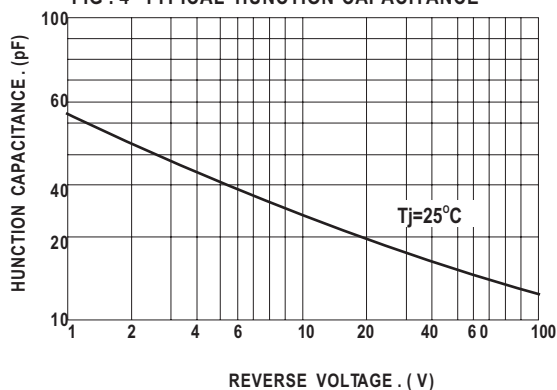
FIG. 4 - TYPICAL HUNCTION CAPACITANCE
