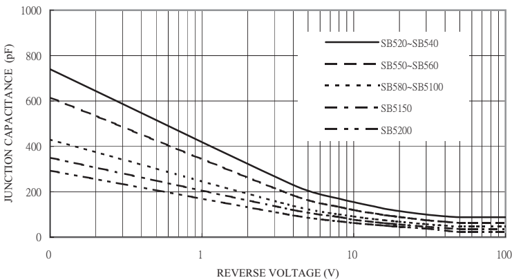
FIG. 4-TYPICAL JUNCTION CAPACITANCE
