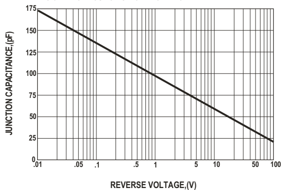
FIG.5-TYPICAL JUNCTION CAPACITANCE
