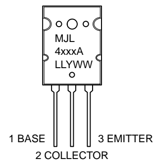
TO-264 CASE 340G STYLE 2
