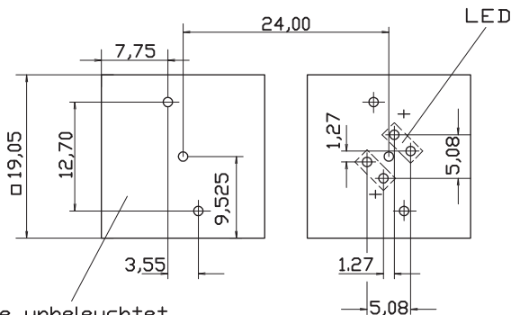
Taste unbeleuchtet keyswitch not illuminated
