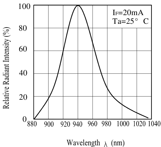
Fig.1 Spectral Distribution
