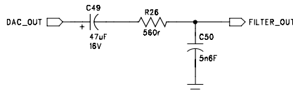
Recommended DAC Output filter - Passive
