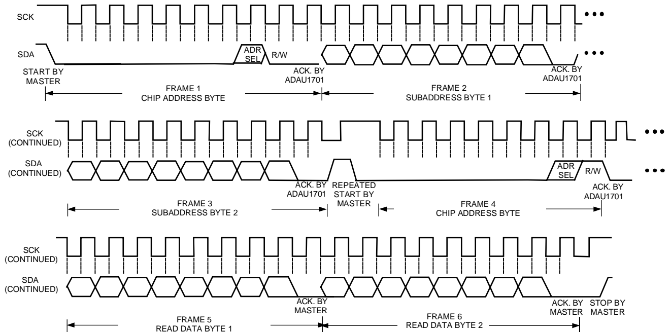
Figure 23. ADAU1701 I2C Read Clocking
