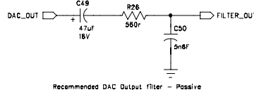
Recommended DAC Output filter - Passive
