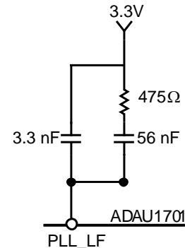
Figure 17. PLL Loop Filter
