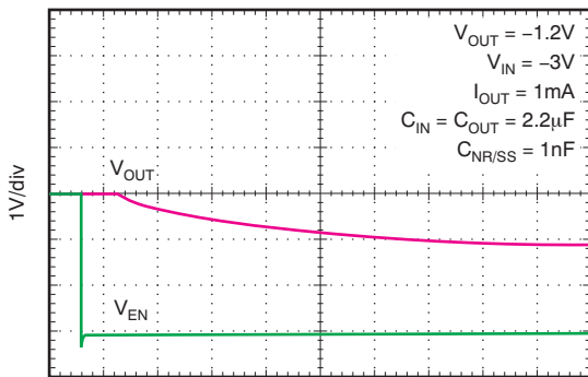
Time (100µs/div)
