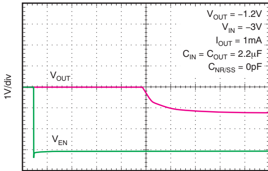
Time (10µs/div)
