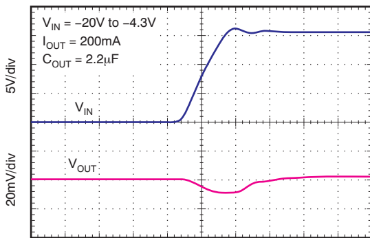
Time (10µs/div)
