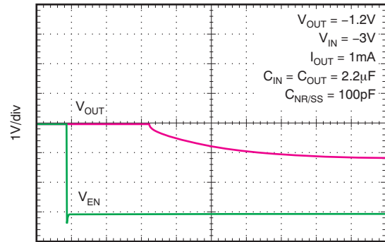
Time (20µs/div)
