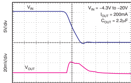
Time (10µs/div)
