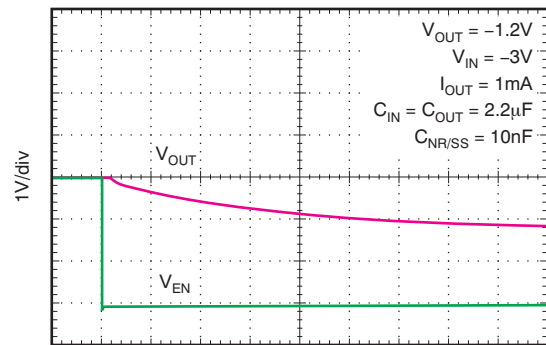
Time (1ms/div)
