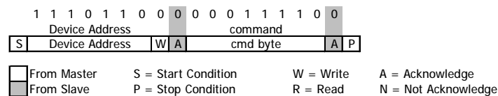
Figure 10: I 2 C Reset Command
