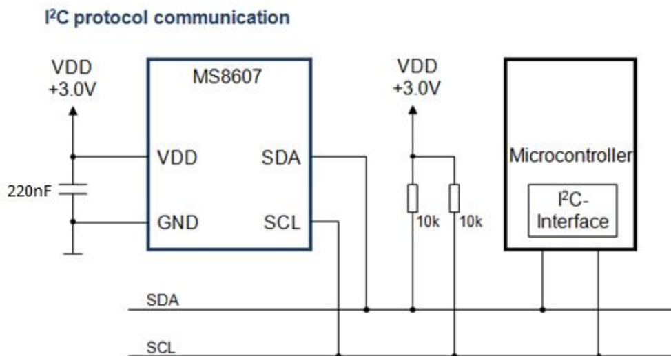
Figure 9: Typical application circuit
