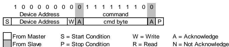
Figure 16: I 2 C Reset Command
