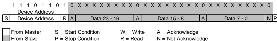
Figure 15: I 2 C answer from the ASIC
