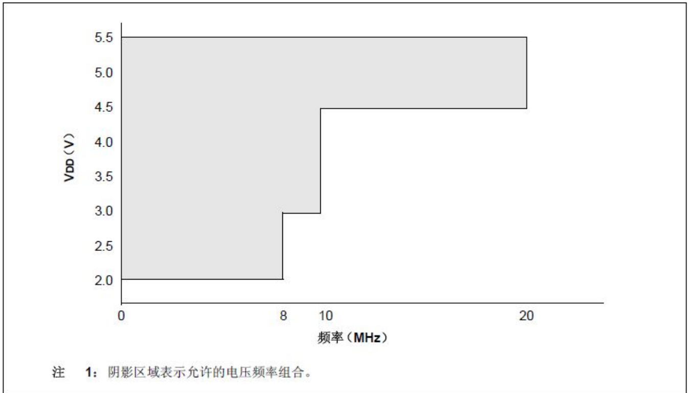
图 13-1-1: EN8F684 电压—频率图, -40^{\circ}\text{C} \leq \text{TA} \leq +85^{\circ}\text{C}
