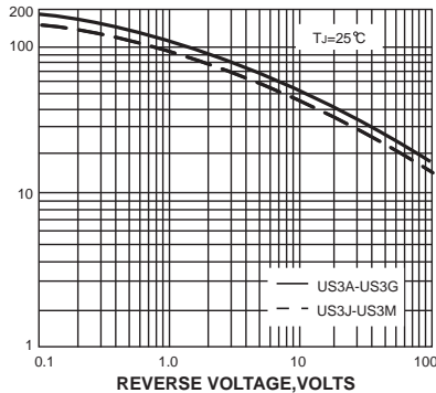
FIG. 5-TYPICAL JUNCTION CAPACITANCE
