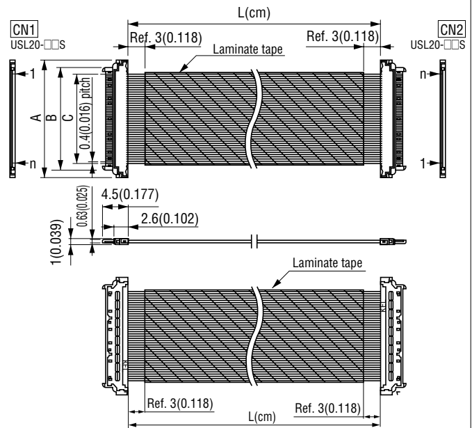
Wiring Code : Pin 1 to Pin n Unit:mm(inch)
