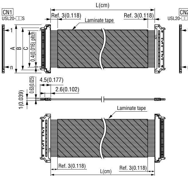
Wiring Code : Pin 1 to Pin 1 Unit:mm(inch)
