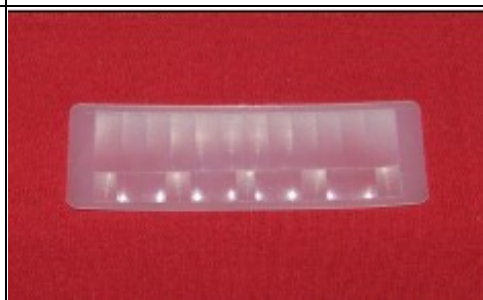
7804-4,尺寸:23.2*56.2mm, 焦距:22mm,角度:70,距离 10m,
