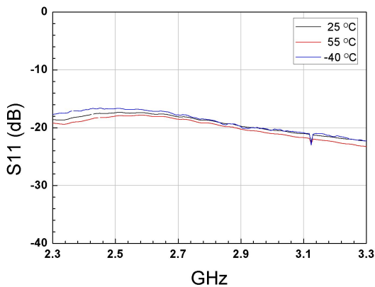
Figure.11 S11 vs Temperature with -10dBm input power
