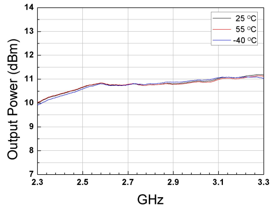
Figure.14 Output Power with -18dBm input power
