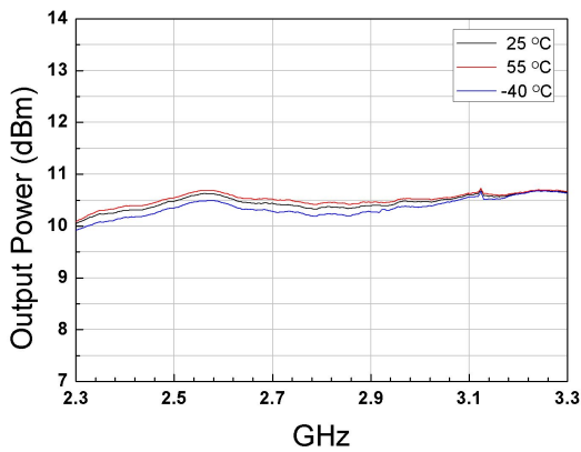
Figure.17 Output Power with -12dBm input power
