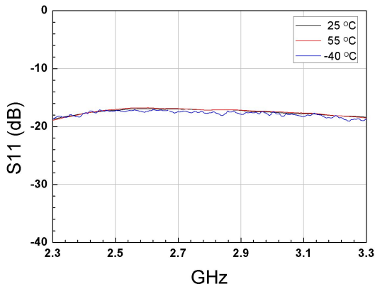
Figure.1 S11 vs Temperature with -20dBm input power
