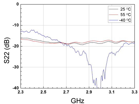
Figure.12 S22 vs Temperature with -10dBm input power
