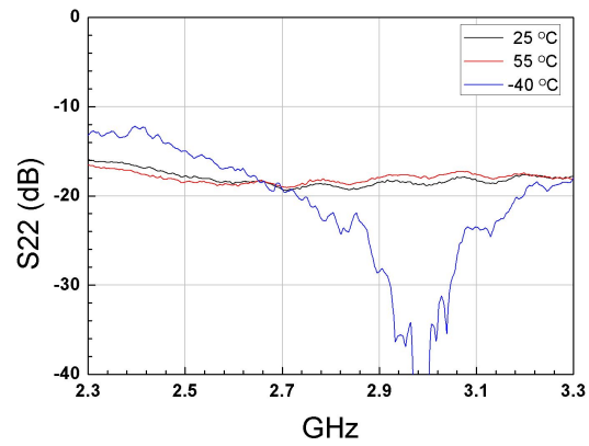
Figure.4 S22 vs Temperature with -18dBm input power
