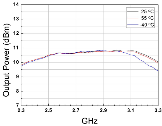
Figure.13 Output Power with -20dBm input power
