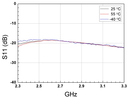
Figure.5 S11 vs Temperature with -16dBm input power
