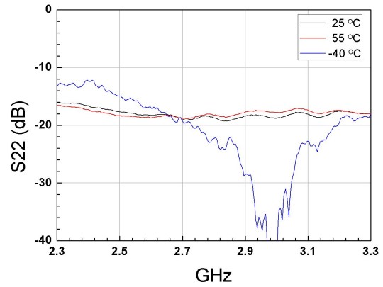
Figure.10 S22 vs Temperature with -12dBm input power
