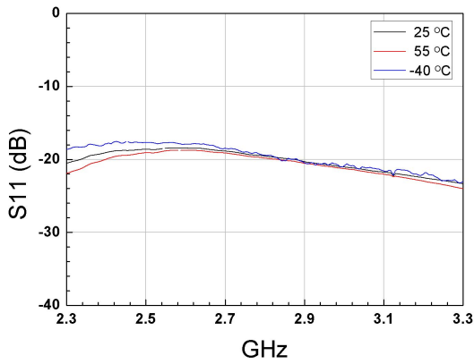
Figure.7 S11 vs Temperature with -14dBm input power
