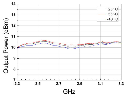
Figure.18 Output Power with -10dBm input power
