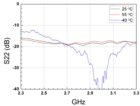
Figure.6 S22 vs Temperature with -16dBm input power
