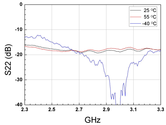
Figure.8 S22 vs Temperature with -14dBm input power
