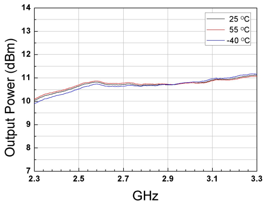
Figure.15 Output Power with -16dBm input power
