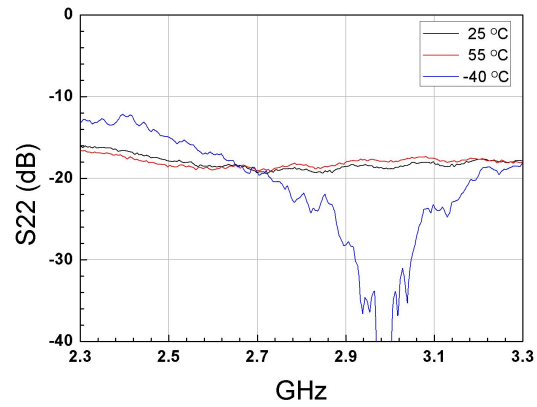
Figure.2 S22 vs Temperature with -20dBm input power
