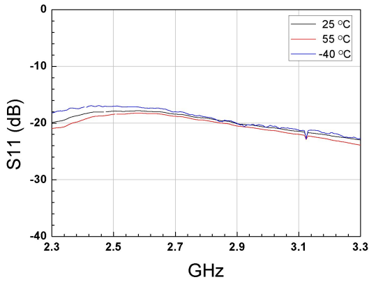
Figure.9 S11 vs Temperature with -12dBm input power
