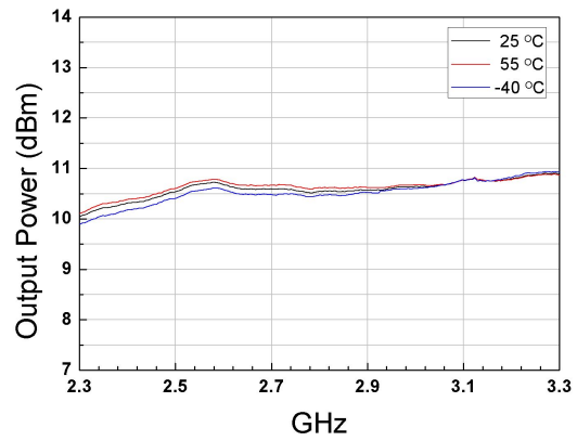
Figure.16 Output Power with -14dBm input power
