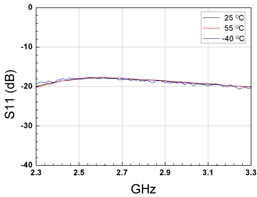
Figure.3 S11 vs Temperature with -18dBm input power
