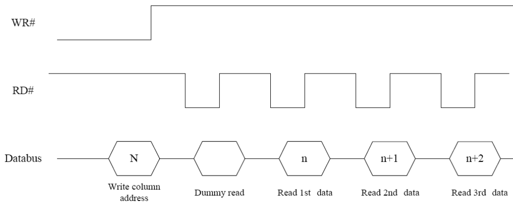
Display data read back procedure - insertion of dummy read
