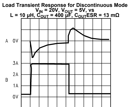
Figure 16. Horizontal Time Base: 1 \mu\text{s}/\text{div}
