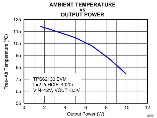
Figure 38. Maximum Ambient Temperature ( f_{SW}=2.5\text{MHz} )
