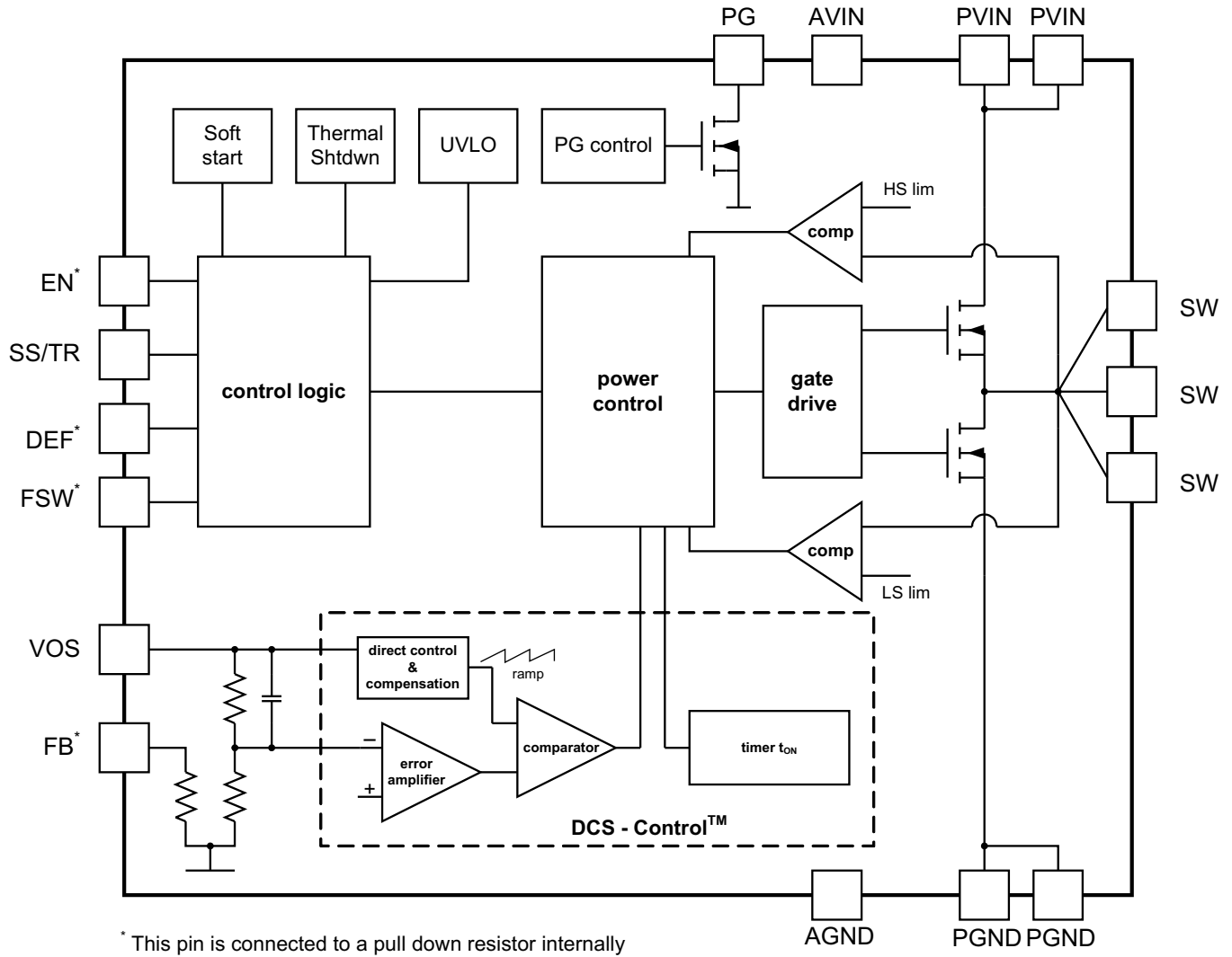
Figure 3. TPS62131/2/3 (fixed output voltage)
