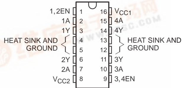
NE PACKAGE (TOP VIEW)
