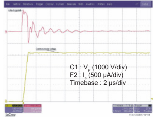
Figure 12: Detail of typical common mode perturbation (4200 V step with 6 kV/ \mu s, R_M = 100 \Omega )
