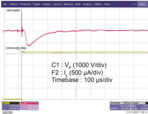
Figure 11: Typical common mode perturbation (4200 V step with 6 kV/ \mu s, R_M = 100 \Omega )
