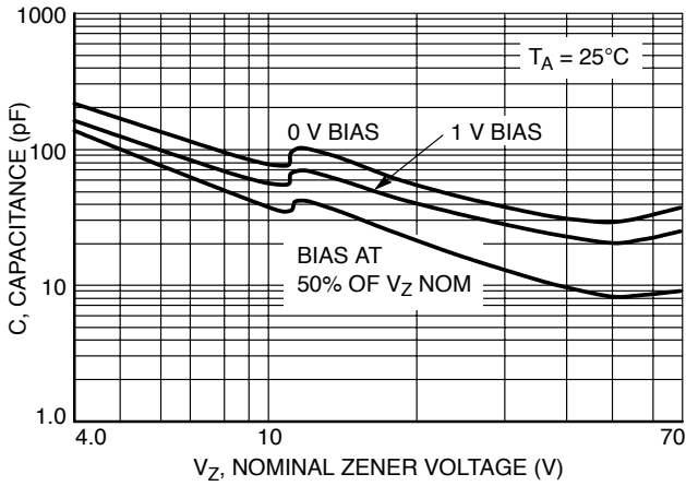
Figure 3. Typical Capacitance
