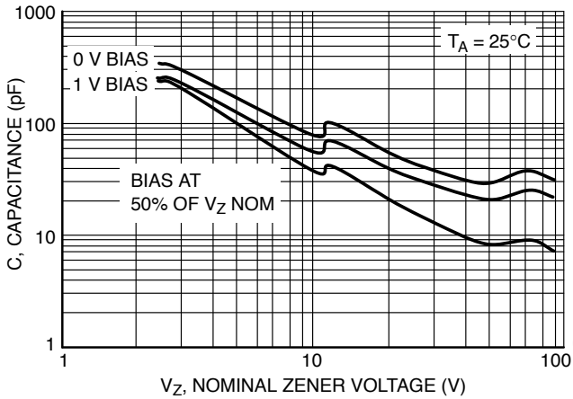
Figure 7. Typical Capacitance
